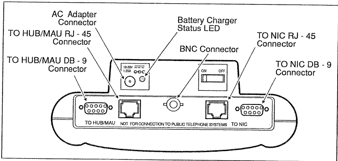
Figure 3-9. Network and AC Adapter Connectors (686/685 Shown)
